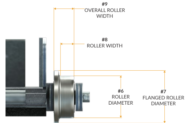
DETAIL C SCALE 1 : 2
