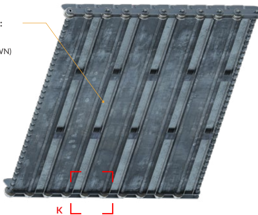
#20 C-CHANNEL SHOWN (COULD BE ANGLE IRON OR FLAT BAR)
